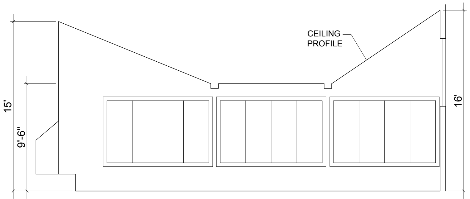
VENTANA BIG SUR FIRESIDE ROOM - BUILDING CROSS-SECTION
